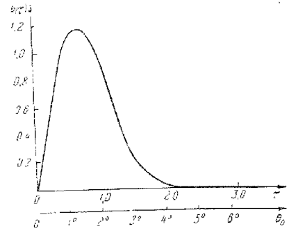
Рис. 20,3. Функция \Phi(\tau) = \sqrt{2\pi} z_0 |G(0, z_0)| ; \tau = \rho^{1/3} z_0 = \left(\frac{\omega}{ca}\right)^{1/3} \sin \theta_0 .
